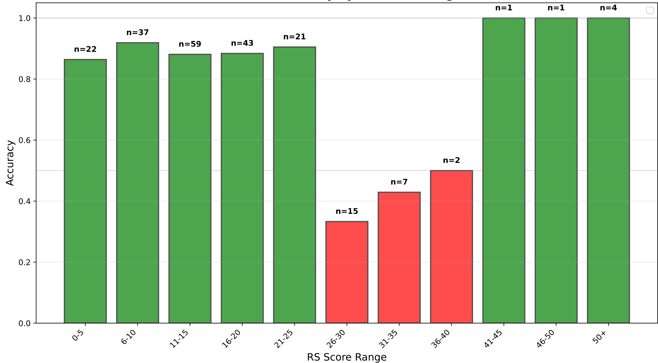
Model Accuracy by RS Score Range
